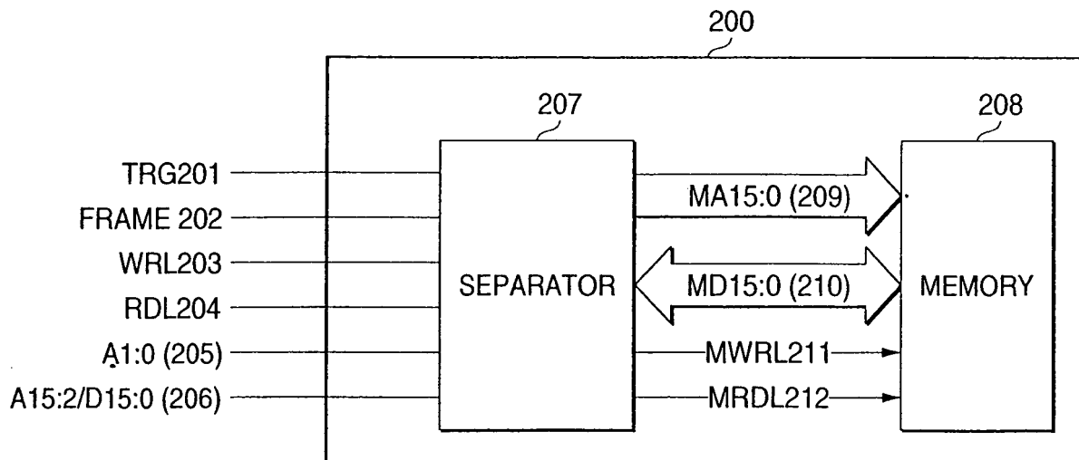
FIG. 17 PRIOR ART
